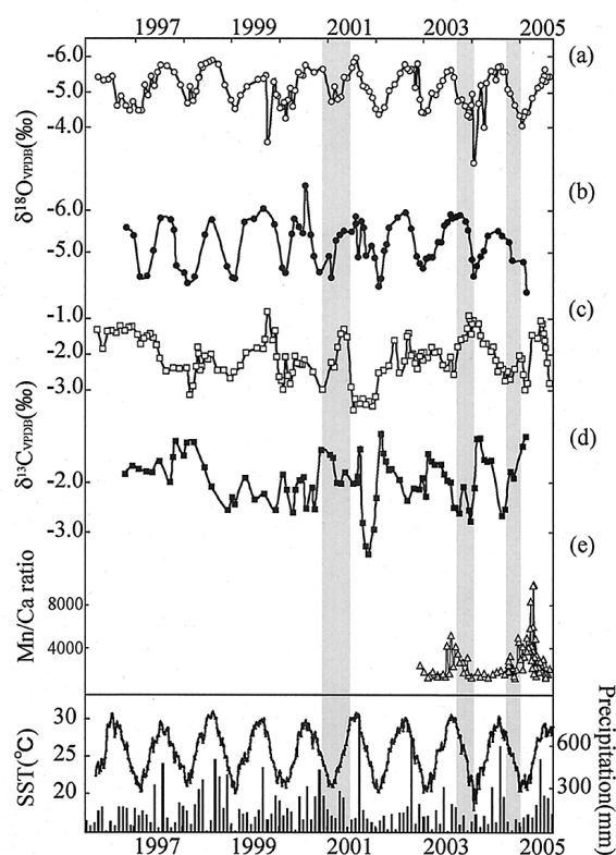
Fig. 5 Time series of geochemical results. Skeletal oxygen isotopic ratio in line A (a) and line B (b). Skeletal carbon isotopic ratios in line A (c) and in line B (d). Skeletal Mn/Ca ratio in line A (e). Also shown are Shiraho SST and precipitation records at Isigaki port (f). Grey areas indicate fluorescence bands observed by fluorescence microscope in coral skeletons.
