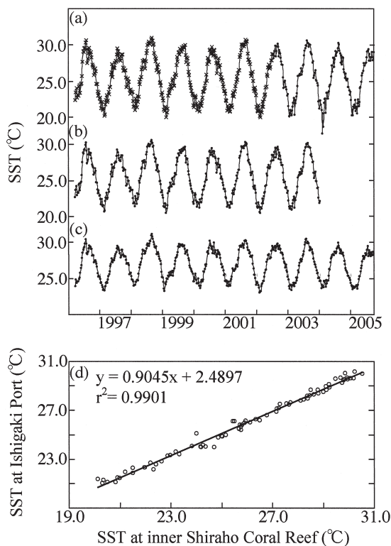
Fig. 3 Time series of sea surface temperature (SST) for Shiraho coral reef (a), Ishigaki port (b), and 1^{\circ} \times 1^{\circ} grid area by the Integrated Global Ocean Services System (IGOSS) (c). Linear relationship between Shiraho SST and Ishigaki port SST from 2002 to 2003 (d). Cross symbols in (a) indicate Shiraho SST calculated from this relationship.
